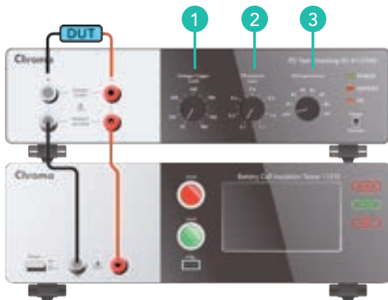
Chroma A112102 connected to Chroma 11210 schematic
