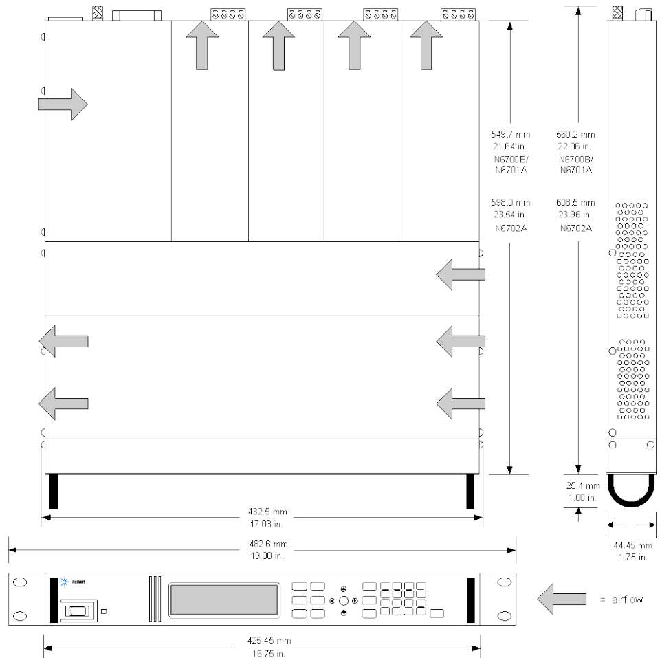
N6731B-N6784A DC Power Modules N6700B-N6705B Mainframes Specifications Guide
