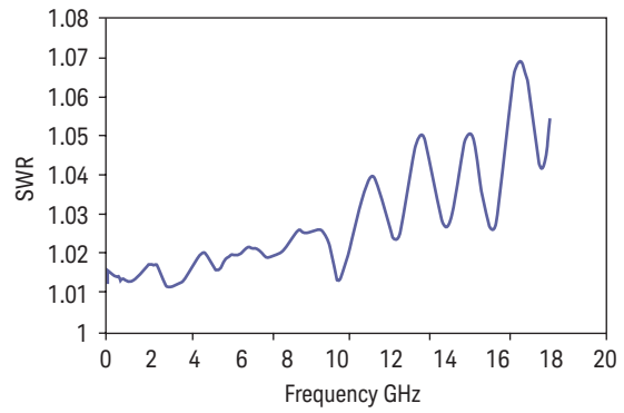
Typical SWR, 10 MHz to 18 GHz ( 25 \pm 10^\circ\text{C} ) for N8481B power sensor
