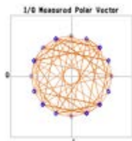
GSM-EDGE constellation (935 MHz carrier)
