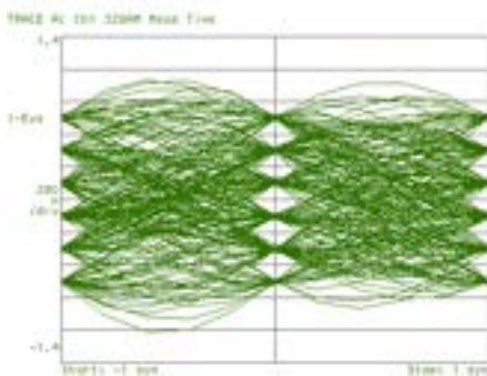
QAM32 I-Eye diagram (5.8 GHz carrier)
